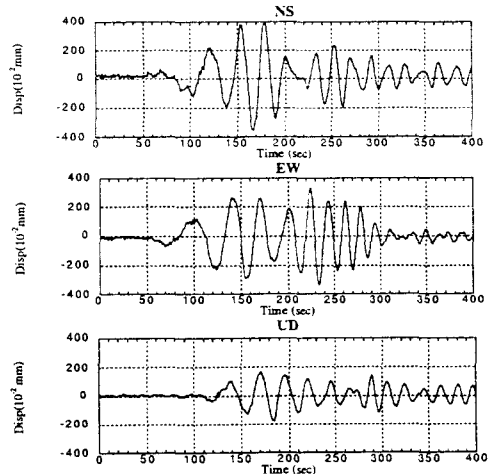
Fig.3 Displacement time histories of Hokkaido Toho Oki earthquake at site D.
