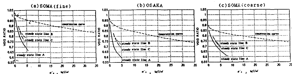
図2 steady-state line A, B, Cと圧密曲線
