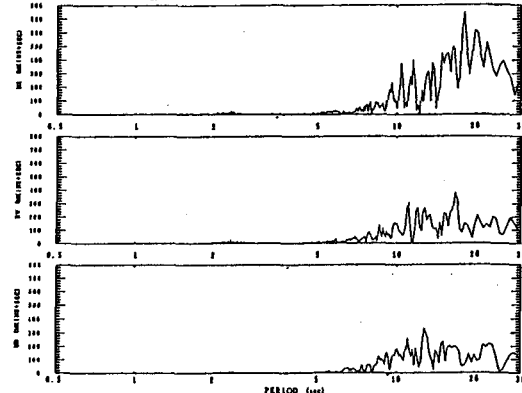
Fig. 3(2) Fourier spectra of Myanmar earthquake velocity record (Tarumi).
