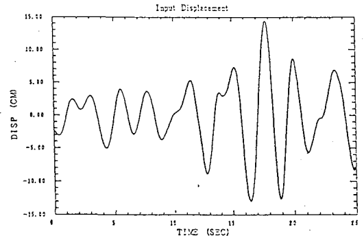
Fig.2 Time Series of Mexico Earthquake SCT Record
