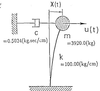
Fig.1 SDOF System Model
