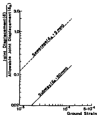
Fig. 7 Response Joint Displacement
