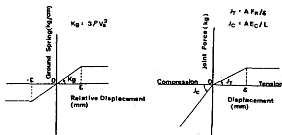
Fig. 3 Ground Spring Fig. 4 Joint
