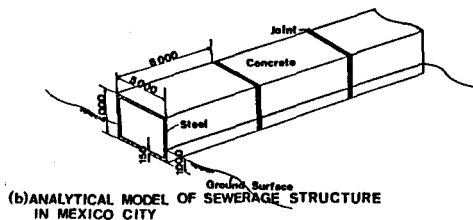
Fig. 2 Analytical Model
