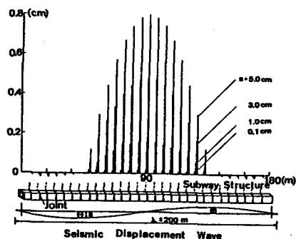
Fig. 5 Joint Expansion and Contraction
