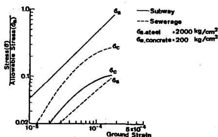
Fig. 6 Response Stress
