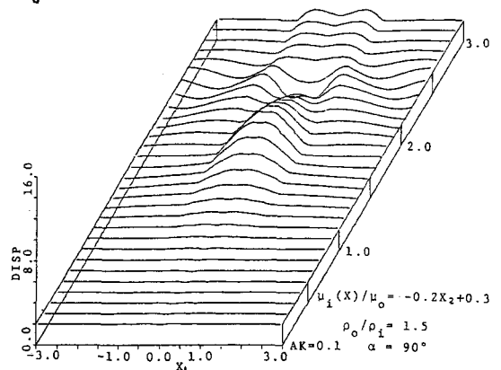
Fig.3 SURFACE-DISPLACEMENT (SEMICIRCLE)
