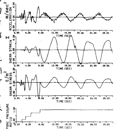
Fig.6 without piles
