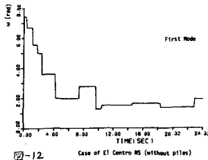
図-12 Case of El Centro 1940 (without piles)
