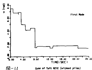
図-11 Case of Taft 1952 (without piles)
