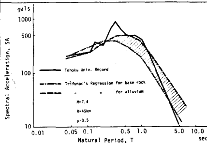
Fig. 2 Tohoku Univ. Spectral Acceleration Record
