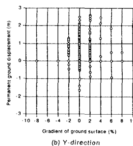
Fig.5 Relationship between gradient of surface and permanent ground displacement.
