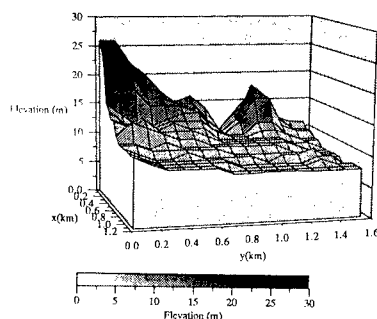
Fig.1 Bird's-eye view of topography.
