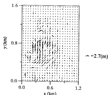
Fig.2 Vector of permanent ground displacement.
