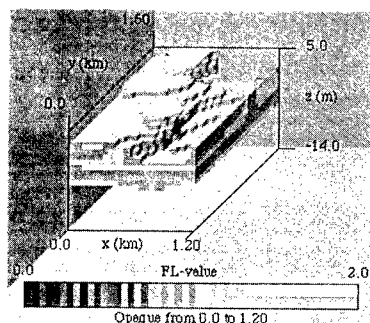
Fig.3 Three-dimensional view of F_L -value.
