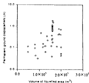
Fig.7 Relationship between volume of liquefied area and permanent ground displacement.
