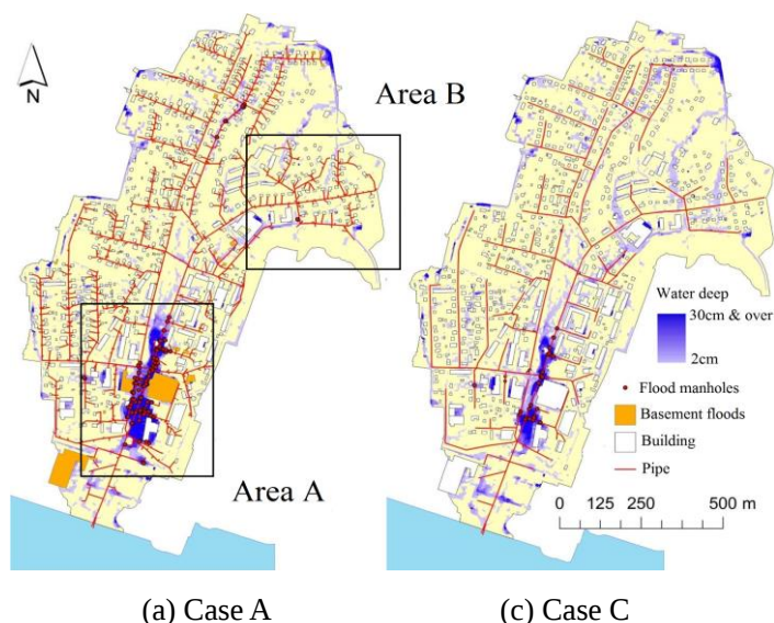
Fig. 2 Maximum flood depths and flood manholes.
