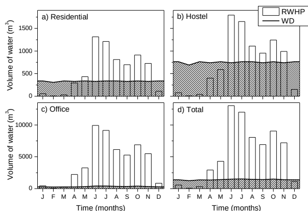
Fig.3 Monthly cumulative rain water harvesting potential (RWHP) and water demands (WD) of (a) residential; (b) hostel; and (c) office buildings; and (d) total of non-agricultural
