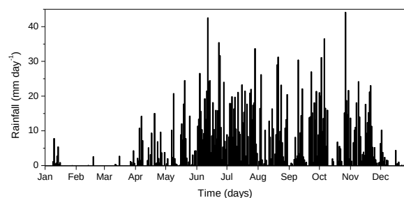
Fig.2 Daily rainfall of the study area during 1 st January to 31 st December, 2010.
