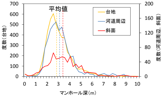
図-6 埋設管路深さの度数分布図
