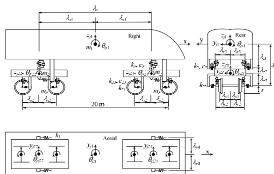
Fig. 2 High-speed train model
