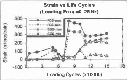
Fig.9 Measured Strain Comparison
