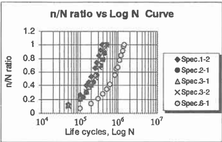
Fig.6 Load Ratio vs Life Cycles Curve
