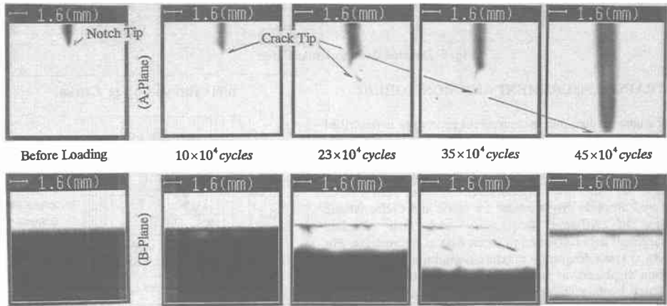
Fig.3 C-scan Images of Specimen No.2-1
