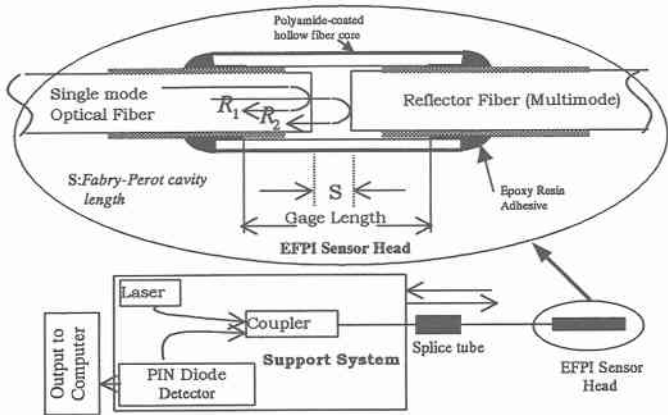
Fig.2 Schematic of the EFPI Sensor and AFSS-PC Support System
