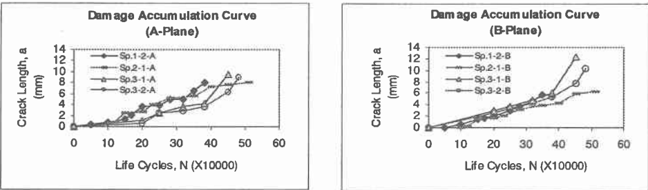
Fig. 5 Damage Accumulation Curve
