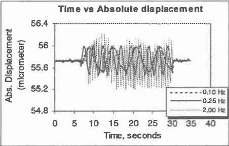
Fig.7 Fatigue Loading Frequency Curve
