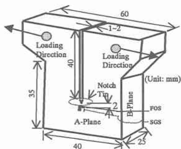
Fig.1 Test Specimen
