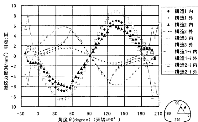
図-8 覆工の縁応力 (せん断変形, \nu=0.30 )
