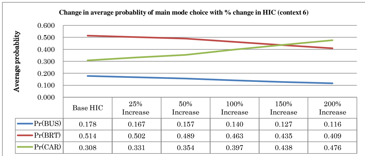
Fig. 15 Sensitivity to change in HIC on main mode choice probability under context 6
