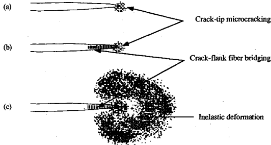
Fig.10 Fracture Failure Mode and Crack Tip Process of Various Cementitious Materials, (a) Neat Cement; (b) Concrete and FRC; and (c) Spectra ECC.
