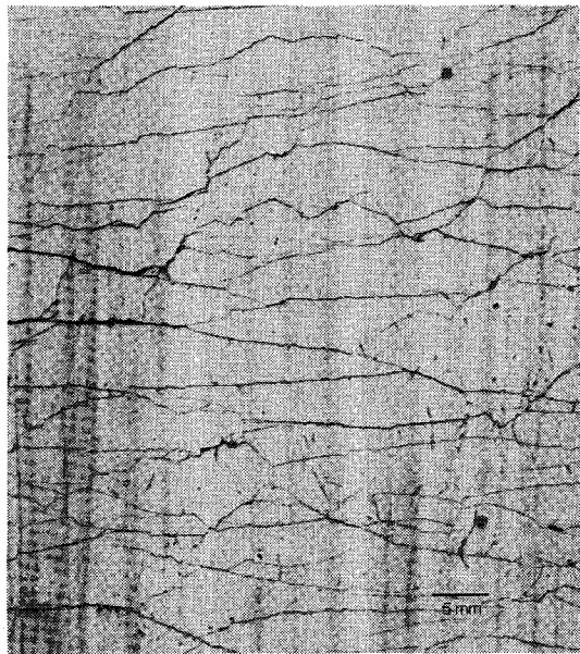
Fig.8 Multiple Cracking in a Spectra ECC ( V_f=2\% ) Uniaxial Tensile Specimen.
