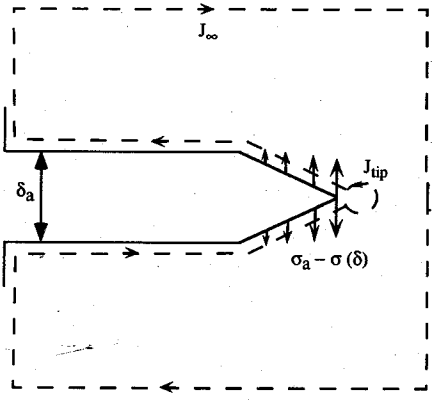
Fig.3 Steady State Cracking (a) Showing Remote Stress, Crack Shape and Traction on Crack; and (b) J-integral Contour on Equivalent Problem (after Marshall and Cox, 1988).
