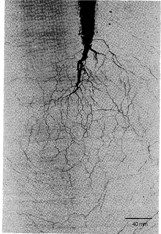
Fig.12 Extensive Damage Development near the Crack Tip in a Spectra ECC ( V_f=2\% ) Fracture Specimen.
