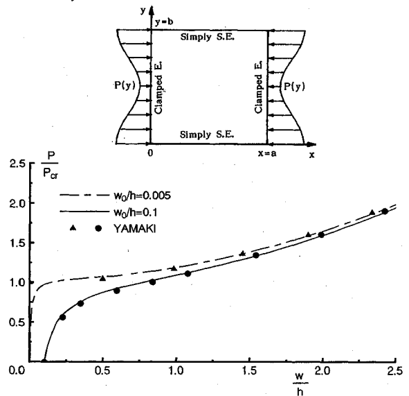
Fig. 13 Load-deflection curves under edge compression (CSCS).
