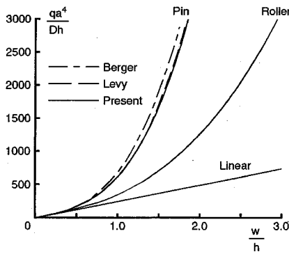
Fig. 6 Load-deflection curves under uniform lateral load (SSSS).
