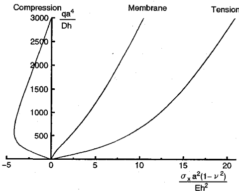
Fig. 8 Load-stress curves under uniform lateral load (roller).
