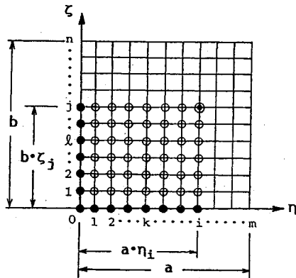
Fig. 2 Discrete points on rectangular plate.
