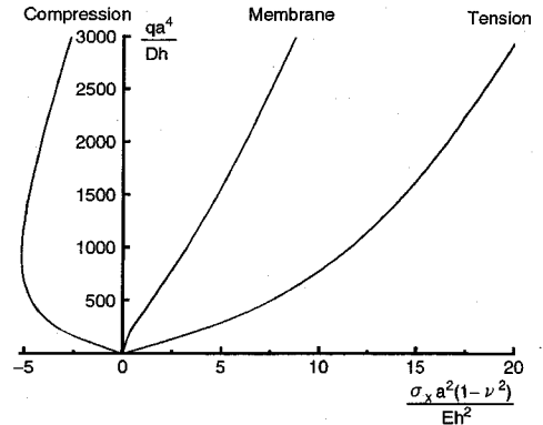
Fig. 10 Load-stress curves under uniform lateral load (SCSC).
