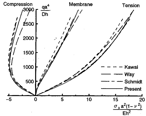
Fig. 5 Load-stress curves under uniform lateral load (CCCC).
