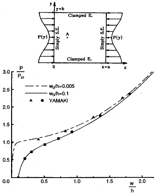
Fig. 14 Load-deflection curves under edge compression (SCSC).
