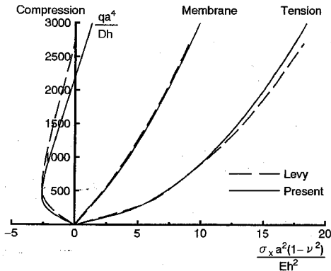
Fig. 7 Load-stress curves under uniform lateral load (pin).
