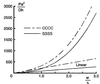
Fig. 11 Load-deflection curves under a concentrated load.
