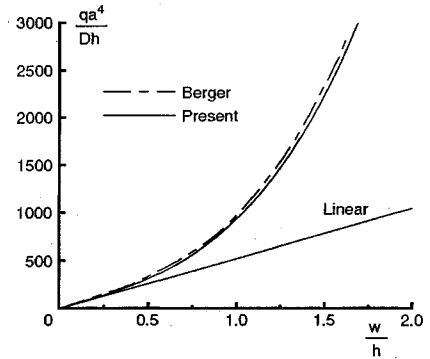
Fig. 9 Load-deflection curves under uniform lateral load (SCSC).
