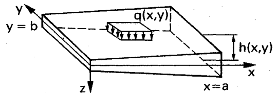
Fig.1 Rectangular plate and coordinate system.
