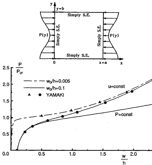
Fig. 12 Load-deflection curves under edge compression (SSSS).
