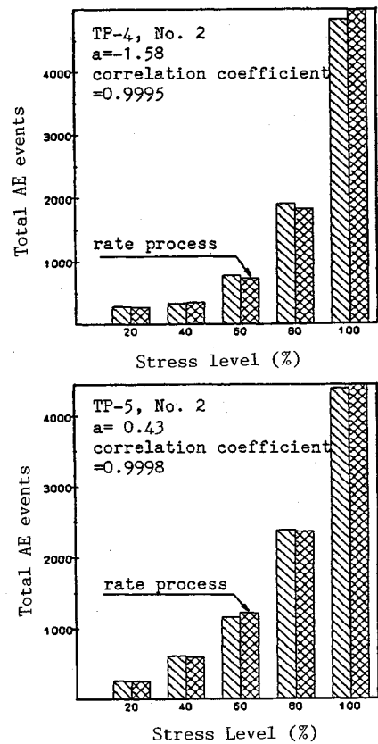
Fig.6 Total AE events versus stress level in core samples.
