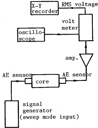
Fig.7 Experimental set up for measuring spectral responses of cores.
