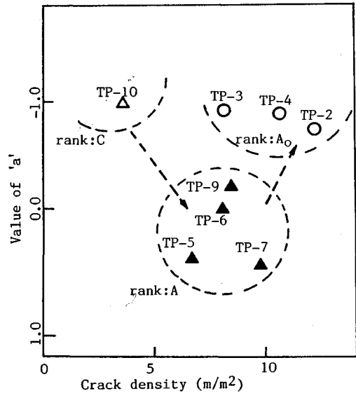
Fig.9 Relations between crack densities of RC slabs and 'a' values in core tests.
