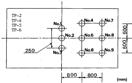
Fig.2 Core-drilled locations in RC slabs.
