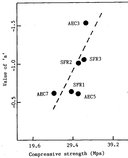
Fig.4 Relations between compressive strengths and 'a' values in newly cast concrete samples.
