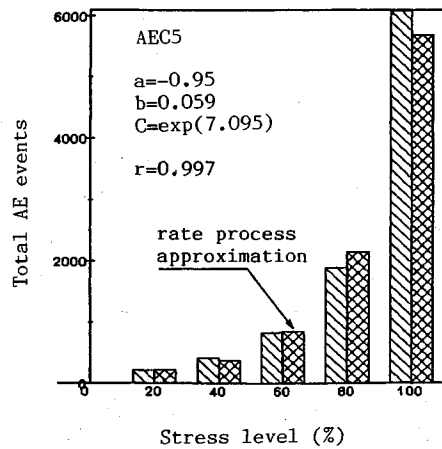
Fig.3 AE activity versus stress level during a uniaxial compression test of AEC5 sample.
