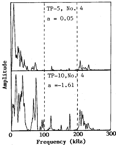
Fig.8 Frequency spectra in core samples.
