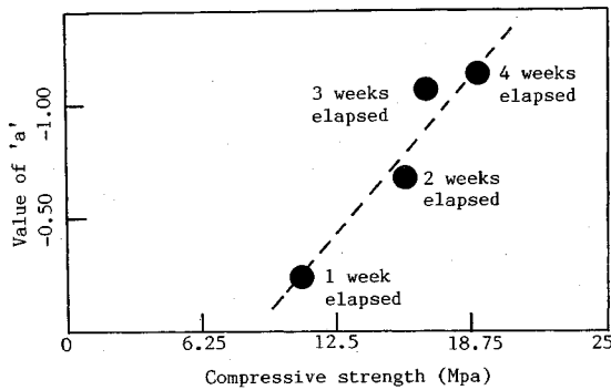
Fig.5 Relations between compressive strengths and 'a' values at the age of one week, two weeks, three weeks, and four weeks elapsed.
