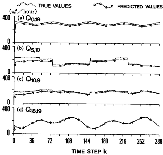
Fig. 5 Results of the one-step ahead prediction for pipe discharges.
