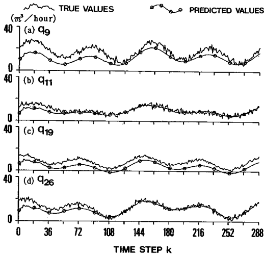
Fig. 4 Results of the one-step ahead prediction for node water demands.
