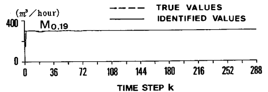
Fig. 9 Identified parameter M_{0,19} for Q_{0,19} when all inflows are observable.
