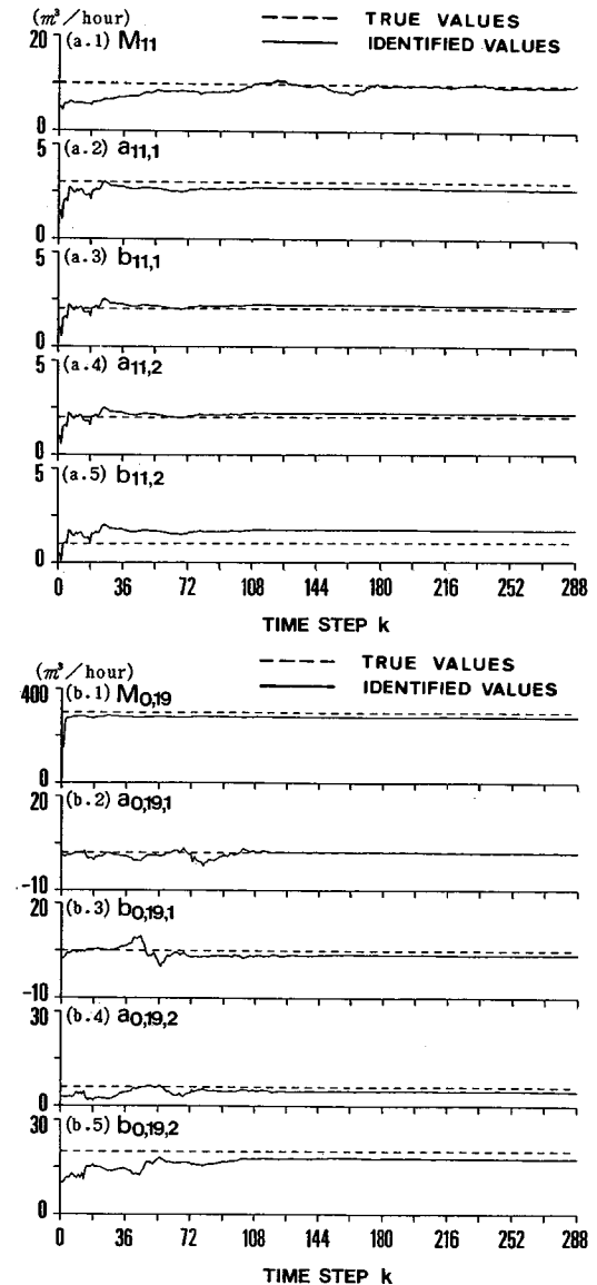
Fig. 7 Identified parameters for q_{11} and Q_{0,19} .
