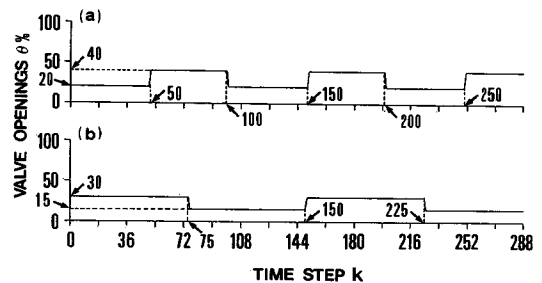
Fig.3 Valve openings used in the simulation.
