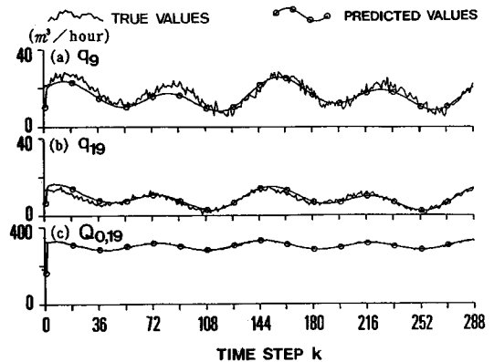
Fig. 8 Results of the one-step ahead prediction of q_9 , q_{19} , Q_{0,19} when all inflows are observable.
