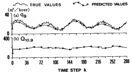
Fig. 10 Results of the one-step ahead prediction of q_9 , Q_{10,9} when a flow meter is set between nodes 9 and 10.
