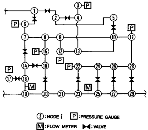
Fig. 2 Block No. 9 of the Fukuoka City water supply network.
