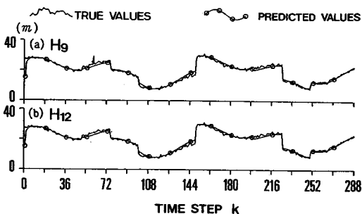
Fig. 6 Results of the one-step ahead prediction for node hydraulic pressures.
