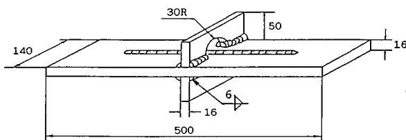
Fig. 1 Specimen (Dimension : mm).
