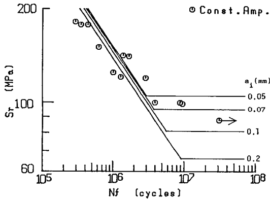
Fig. 11 Estimated S_r-N_f Curves under Constant Amplitude Loading.
