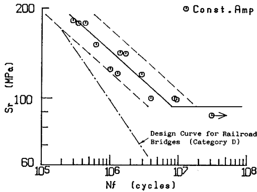
Fig. 4 S_r-N_f Relationships under Constant Amplitude Loading.
