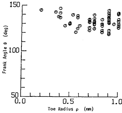
Fig.9 Measured \theta and \rho .
