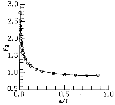
Fig.10 Relationship between F_g and a/T .
