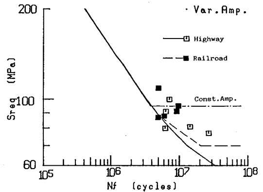
Fig. 12 Estimated S_{req}-N_f Curves under Variable Amplitude Loading.
