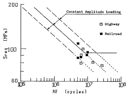
Fig. 6 S_{req}-N_f Relationships under Variable Amplitude Loading.
