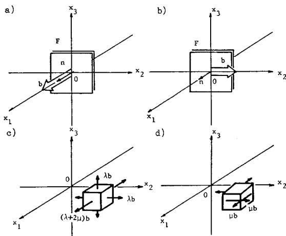
Fig. 6 a) A dislocation model for a tensile crack and b) that for a shear crack on the crack surface. c) Normal components for a tensile crack and d) corresponding off-diagonal components for a shear crack.
