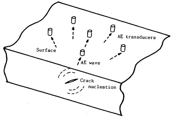
Fig.2 A multi-channel AE observation of crack nucleation.
