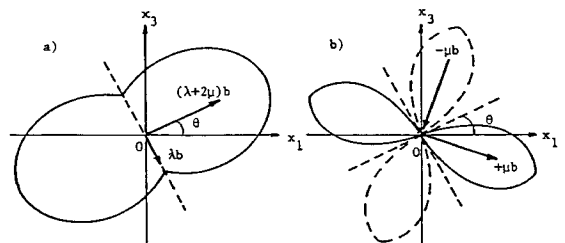
Fig. 7 a) The radiation pattern of P wave due to a tensile crack and eigenvectors with the magnitude of eigenvalues. b) The radiation pattern of P wave due to a shear crack and eigenvectors with the magnitude of eigenvalues.
