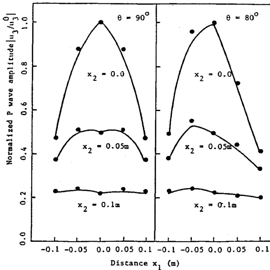
Fig. 9 Solid curves show the first motions in a half space due to tensile cracks. Solid circles indicate those in an infinite space, which are calibrated by the reflection coefficient.
