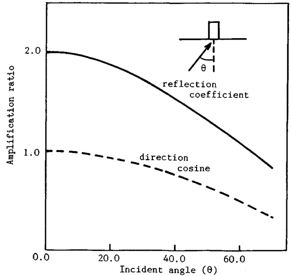
Fig. 10 Comparison between the reflection coefficient and the direction cosine for various incident angles.
