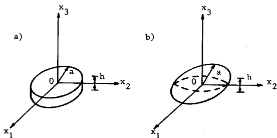
Fig. 3 a) A disk-shaped crack model. b) A penny-shaped crack model.
