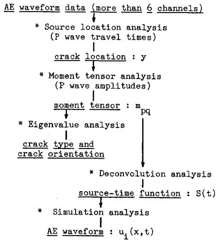
Fig.1 A source inversion procedure proposed for AE waveforms.
