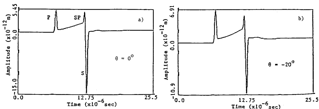
Fig. 5 Simulated AE waveforms due to tensile penny-shaped cracks of a) the case \theta=0^\circ and b) \theta=-20^\circ .
