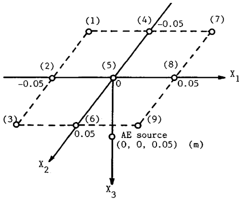
Fig. 11 AE sensor locations assumed in numerical experiments.
