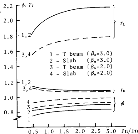
Fig.1 P_n/D_n v.s. \phi , \gamma_i (R.C. Bridge).
