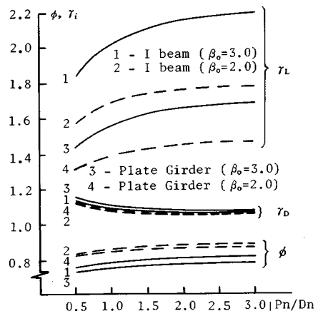
Fig.2 P_n/D_n v.s. \phi , \gamma_i (Steel Bridge).
