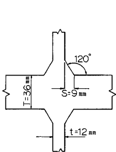
Fig. 4 Standard Size of Welded Joint.
