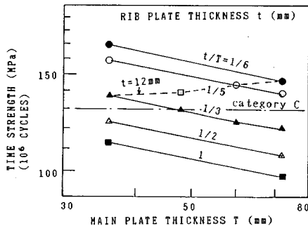
Fig. 5 Effects of Main Plate Thickness and Rib Plate One on the Fatigue Strength.
