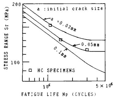
Fig. 3 Predicted S_r-N_p Relations and Test Results.
