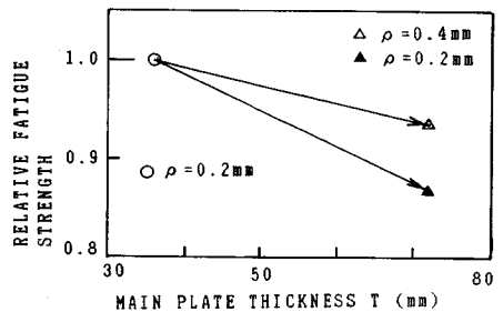
Fig. 6 Influence of Toe Radius on Effects of Thickness.
