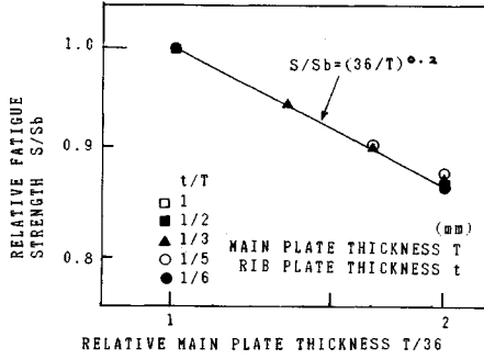
Fig. 7 Effects of Main Plate Thickness on the Fatigue Strength.
