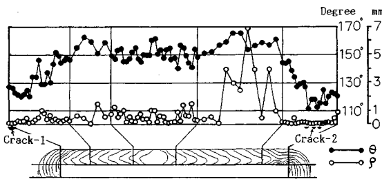
Fig. 1 Flank Angle and Redius at Weld Toe of HC-1 Specimen.
