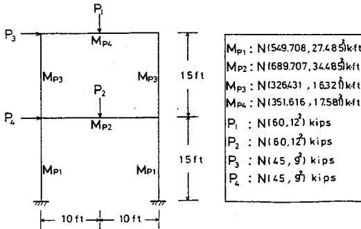
Fig. 3 Example 1 : 2-Story 1-Span Frame.
