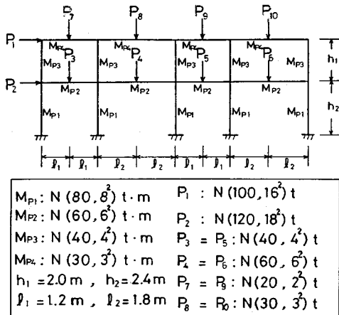
Fig. 6 Example 2 : 2-Story 4-Span Frame.
