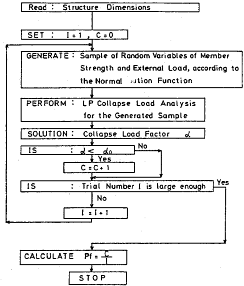
Fig.2 Revised Monte Carlo Simulation.
