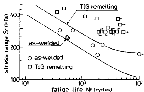
Fig. 13 Predicted S_r-N_f Relationships and Test Results.
