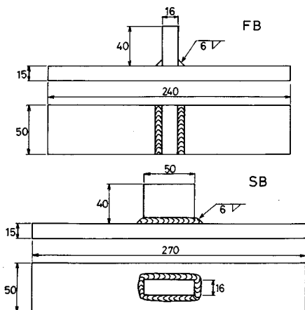
Fig. 1 Configurations and Dimensions of Specimens.
