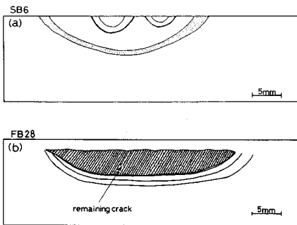
Fig. 11 Beach Marks on Failure Surfaces of Retrofitted Specimens. (a) crack was completely fused, (b) crack was not successfully fused
