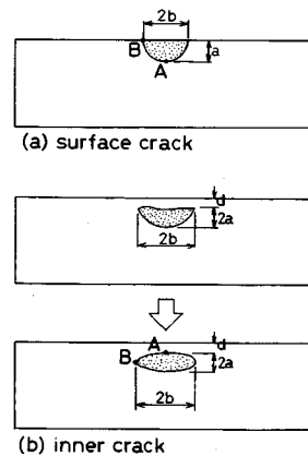
Fig. 12 Simplification of Fatigue Crack for Calculation of Stress Intensity factor.
