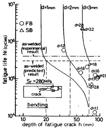
Fig. 14 Predicted Fatigue Life of Joints with Remaining Crack (under Bending).
