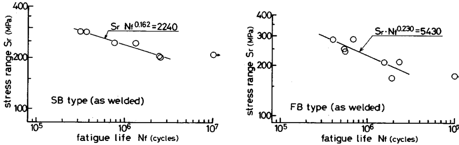
Fig. 6 Fatigue Test Results of As-Welded Specimens.
