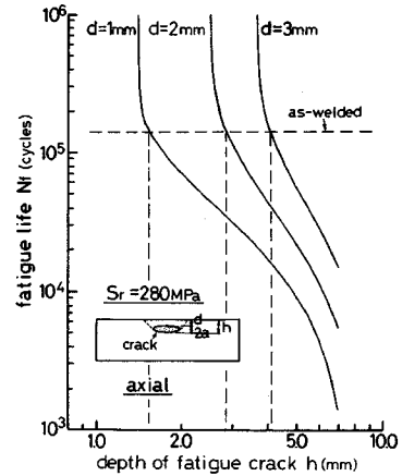
Fig. 15 Predicted Fatigue Life of Joints with Remaining Crack (under Axial Force).
