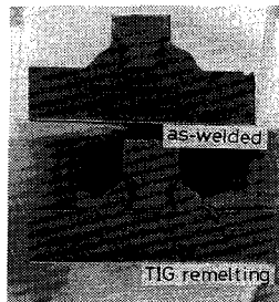
Fig. 4 Macroscopic Photographs of the Fillet Weld Toes.
