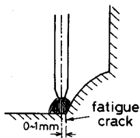
Fig. 3 Position Aimed at by TIG Arc Remelting.
