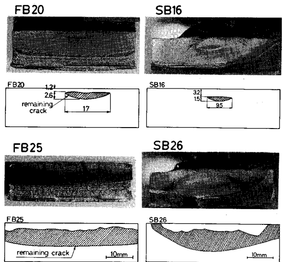
Fig. 10 Failure Surfaces of Retrofitted Specimens.
