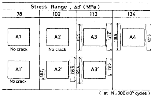
Fig. 4 Fatigue Cracks Originated along Weld Toe.
