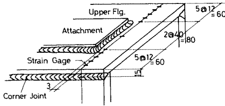
Fig. 16 Location of Strain Gages.
