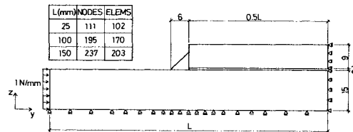
Fig. 13 Model of Finite Element Method.
