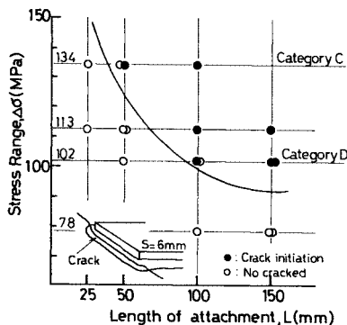
Fig. 10 Influence of Attachment Length.
