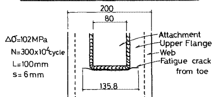
Fig. 7 Appearance of Typical Crack (B3).
