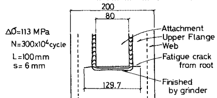
Fig. 5 Appearance of Typical Crack (A2).
