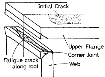
Fig. 19 Fatigue Crack along Root of Corner Weld.
