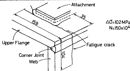
Fig. 18 Fatigue Crack Propagating into Web Plate.
