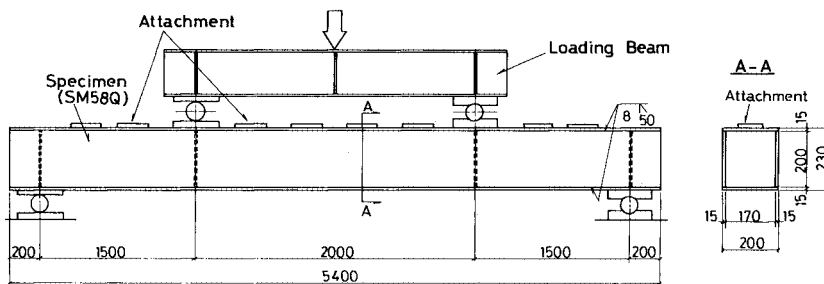
Fig. 1 Configuration and Dimension of Specimen.
