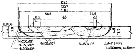
Fig. 6 Fracture Surface of Toe Crack (A3).
