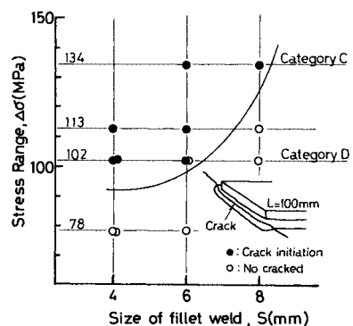
Fig. 11 Influence of Fillet Weld Size.
