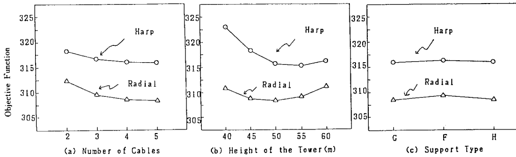
Fig. 11 The Influence on Obj. Function by Parameters.
