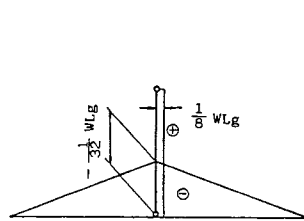
Fig.4 Cross-sectional forces caused by prestress.
