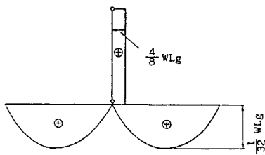
Fig.3 Cross-sectional forces computed from geometrical compatibility.
