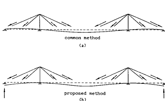
Fig. 7 A method of prestressing for cable-stayed bridge.
