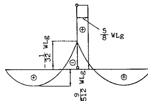
Fig.2 Cross-sectional forces determined to minimize a objective function.
