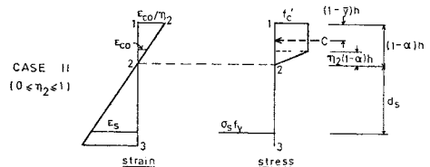
Fig. 5 Strain Compatibility.
