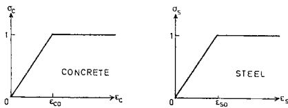
Fig. 3 Stress-strain Relations for Concrete and Steel.
