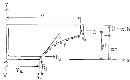
Fig. 2 Collapse Mechanism for Analysis.
