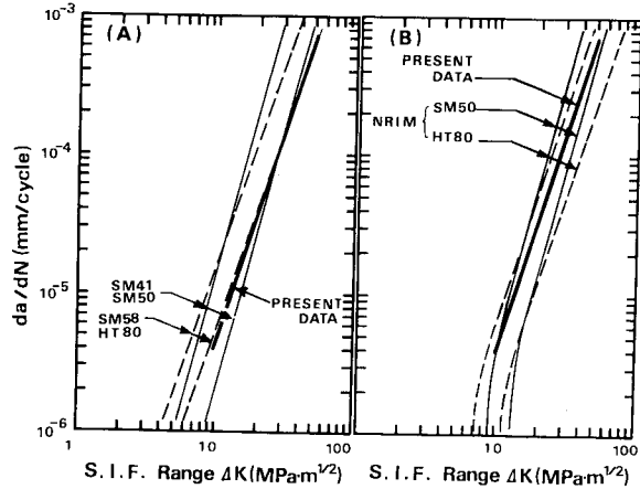
Fig.6 Comparison of constant amplitude fatigue crack growth rates with previous investigations.
