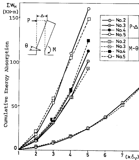
Fig.12 Cumulative energy absorption by load-displacement and moment-rotation relationship.
