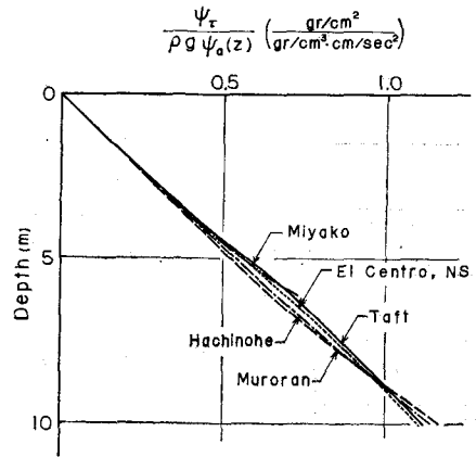
Fig. 10 Stress Distributions
