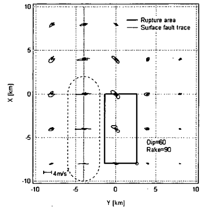
Fig.4 Acceleration trajectories for the mechanism of (dip=60°, rake=90°).
