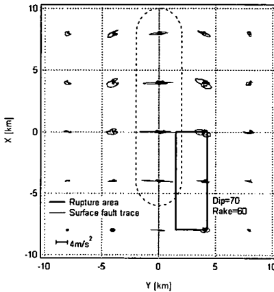
Fig.6 Acceleration trajectories for the mechanism of (dip=70°, rake=60°).
