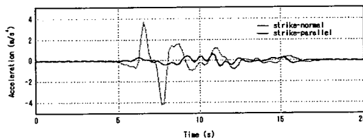
Fig.11 Typical examples of strike-normal (broken line) and strike-parallel (solid line) simulated accelerations (dip=60°, rake=90°, X=0km, Y=-4km).
