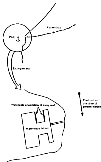
Fig.1 Preferable orientation of important quay walls.
