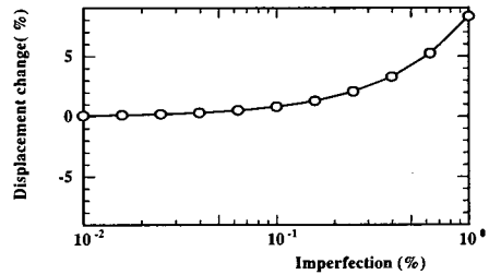
Fig. 8 Displacement & imperfection amplitude relationship
