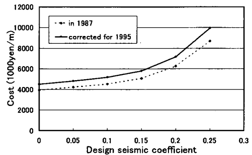
Fig. 12 Construction cost increase due to seismic coefficient increase
