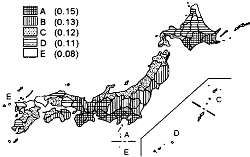
Fig. 7 Regional design seismic coefficient definition for Japanese ports 1)
