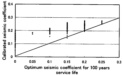
(b) 50% occurrence probability for 100 years
