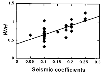
Fig. 2 Correlation between the width to height ratio ( W/H ) and seismic coefficient of a gravity type quay wall 9)
