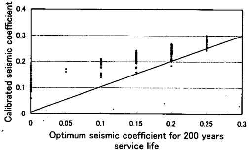
(c) 50% occurrence probability for 200 years
