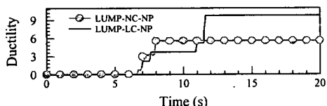
Fig. 8 Ductility at pile top with maximum bending moment.
