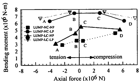
Fig. 5 Bending moment-axial force relationship at pile top when the respective pile attains the maximum bending moment.
