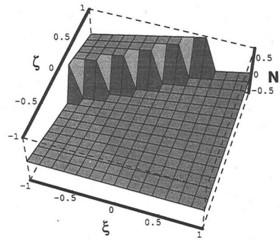
Fig. 5 Shape functions corresponding to crack opening displacements
