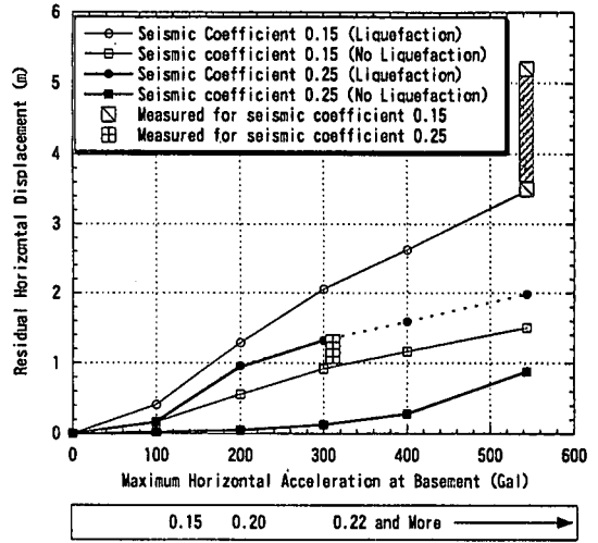
Fig.21 Horizontal displacement under various input acceleration levels.
