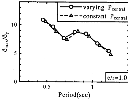
Fig.A2 Comparison of response spectra with the major parameter of e/r
