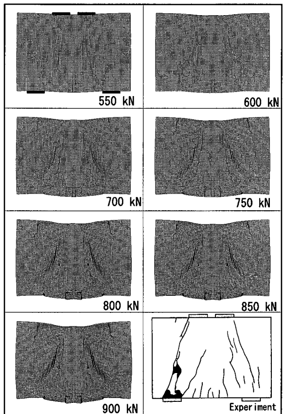
Fig.15 Deformed shape and crack pattern of deep beam (illustration scale factor=40)
