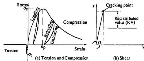
Fig. 2 Tension, compression and shear models for concrete
