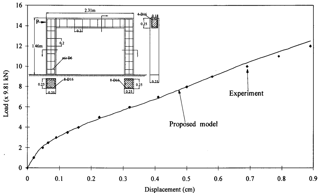
Fig. 12 Load-displacement relation of RC frame
