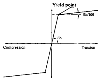
Fig. 3 Stress-strain relation for steel
