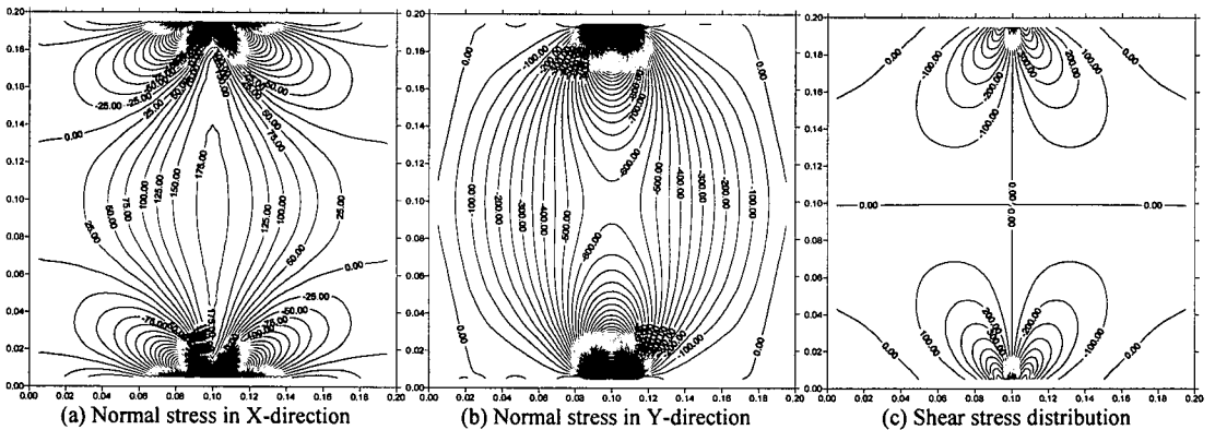
Fig. 7 Stress contours for a concrete cube subjected to concentrated loads (Dimensions are in meters and stresses, x 10kN/m 2 ) (All contours are draw at load-level 120 kN in Case (1), before cracking occurrence)
