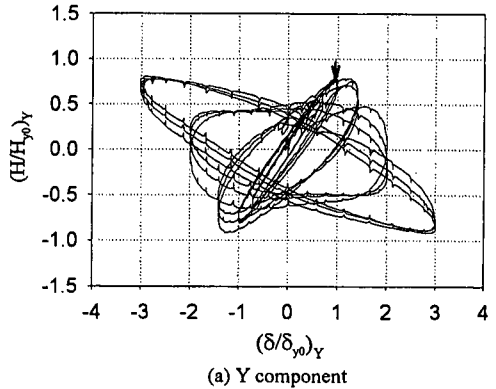
Fig. 11 Normalized lateral load-displacement response in Biaxial-Circular direction (S-BC)
