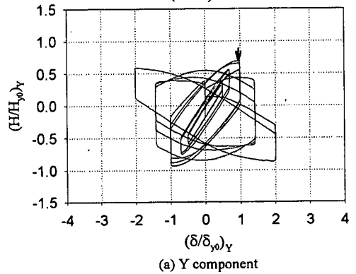
Fig. 10 Normalized lateral load-displacement response in Biaxial-Square direction (S-BS)
