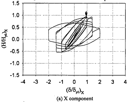
Fig. 10 Normalized lateral load-displacement response in Biaxial-Square direction (S-BS)
