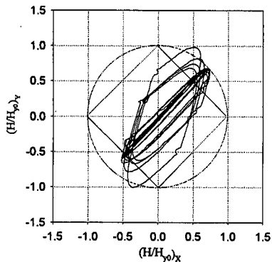
(a) Load path
