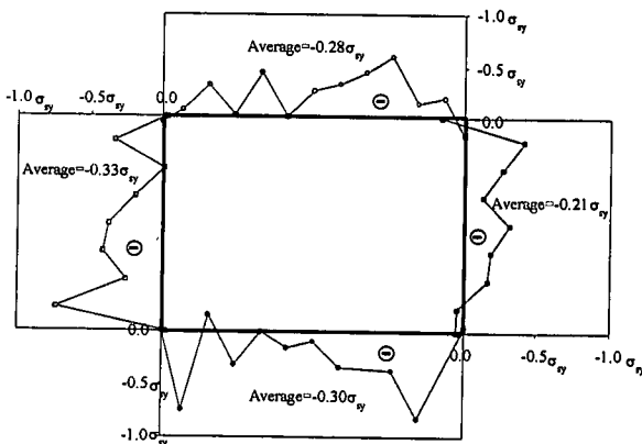
Fig. 6 Distribution of residual stresses
