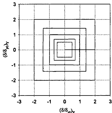
(b) Displacement path
