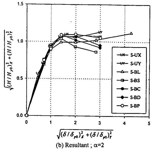
Fig. 20 Resultants and summations of load-displacement response
