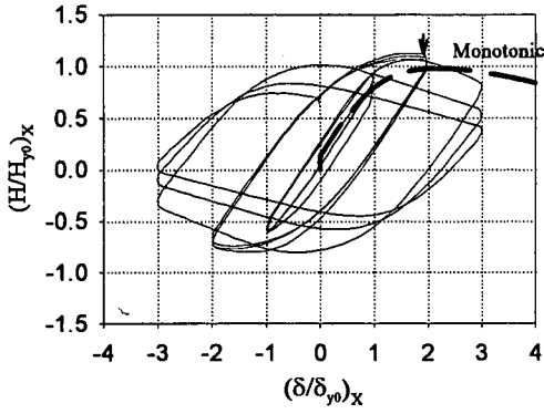
Fig. 7 Uniaxial-X direction (S-UX)
