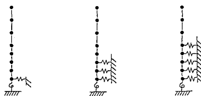
(a) CASE3-90-1 (b) CASE3-90-2 (c) CASE3-90-3
