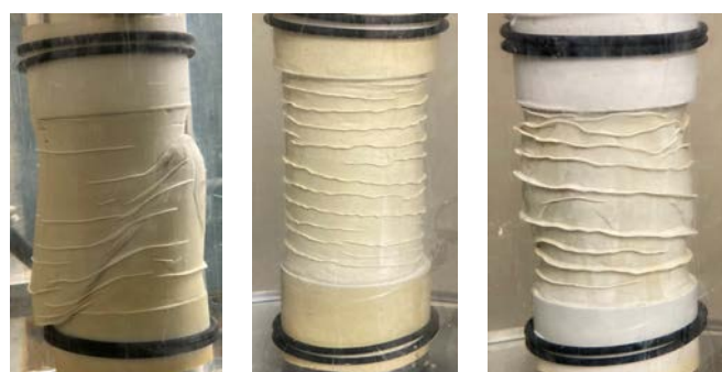
(a) 溶脱なし (b) 溶脱 60min (c) 溶脱 2day
