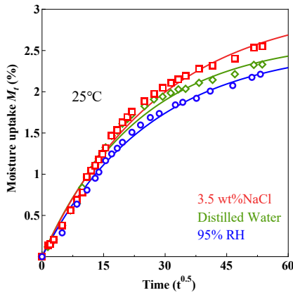
Fig.2 Moisture uptake curve
