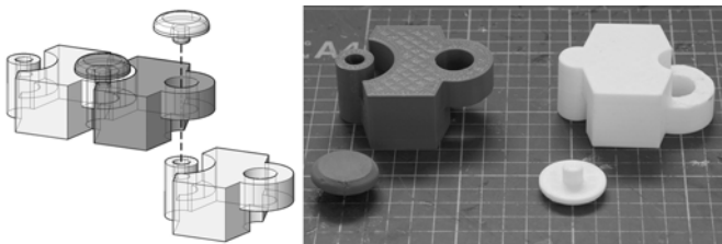
Fig. 1 Left: CAD drawing of two modules linked together and exploded view showing the connection. Right: top and bottom of the 3D-printed prototype.
