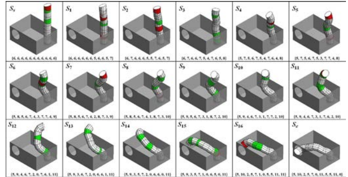
Fig. 4 Transition for Arm-Z found by Particle Swarm Optimization.
