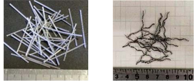
Fig. 1 Used fibers
