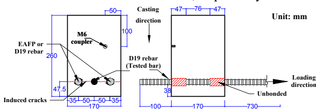
Fig. 1 Specimen detail
