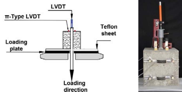
Fig. 2 Loading and measurement of pull-out test
