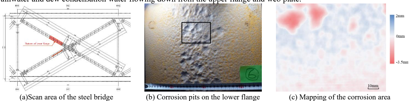
Fig.1 Corrosion pits of weathering steel structure
