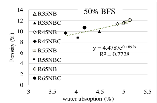
Figure 5. Porosity against water absorption
