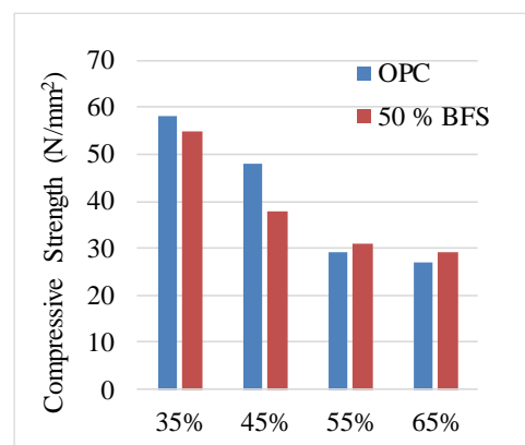
Figure 1. The 28 days' compressive strengths of original concrete.
