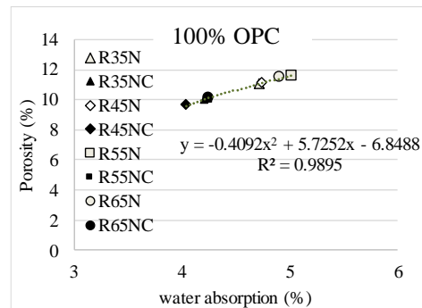
Figure 4. Porosity against water absorption
